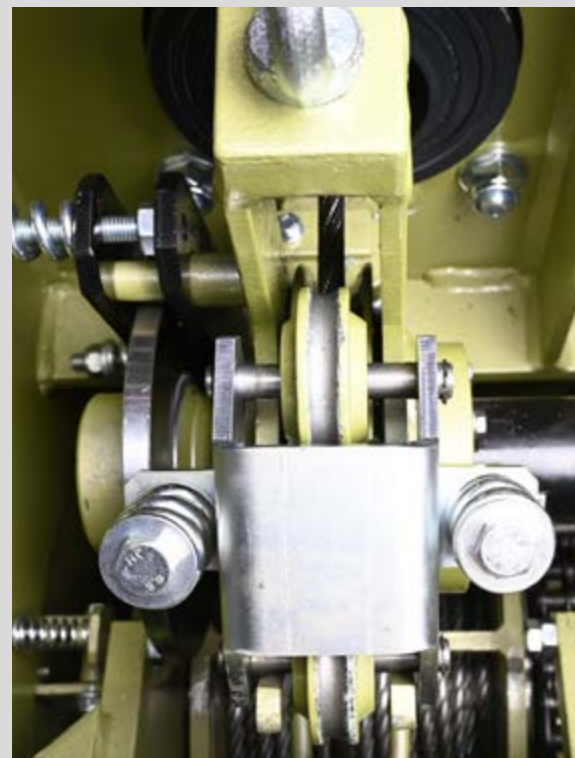
Hydraulic cable ejector with cable dispenser
